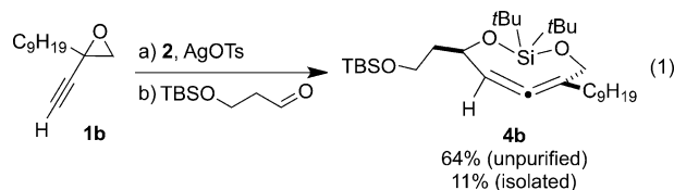
Scheme 1. Insertion of a silylene into a propargylic carbon–oxygen bond and subsequent aldehyde addition. TBS = tert -butyldimethylsilyl, Ts = 4-toluenesulfonyl.
